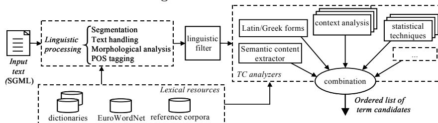
Fig. 2. Architecture of Yate.
